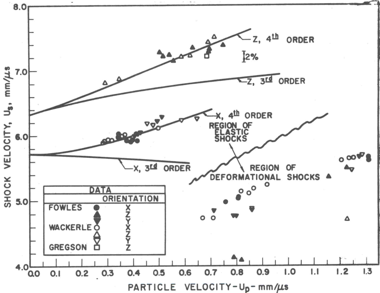
Fig. 2.6.--Shock Velocity as Function of Particle Velocity. Curves labelled 3rd, 4th, are fits based on zero-pressure elastic constants up to 3rd and 4th order respectively for X and Z-cut crystals.
